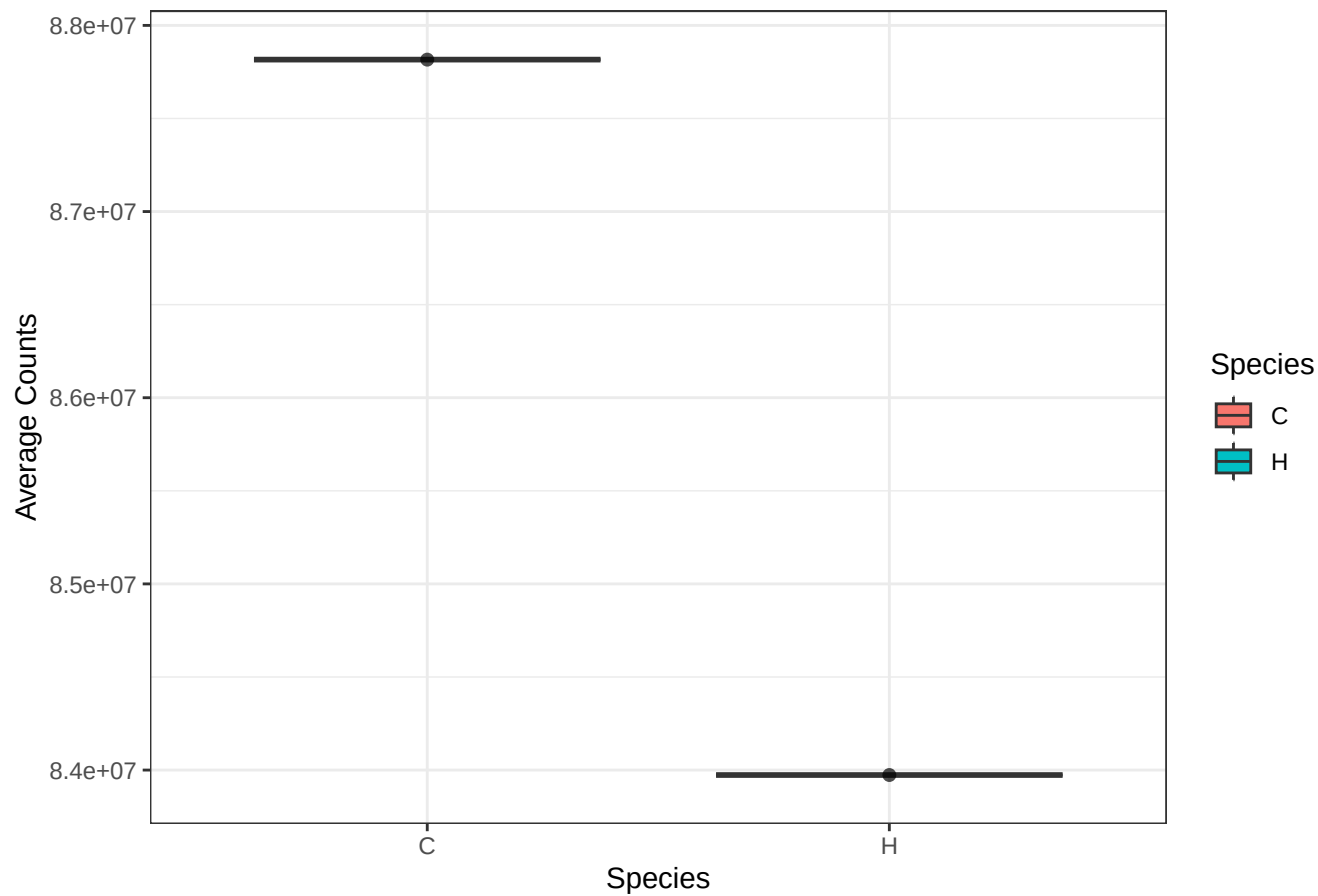
Average Mapped Reads across Species
